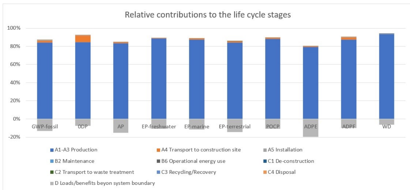
Figure 1: Environmental impacts of door closers along its life cycle
